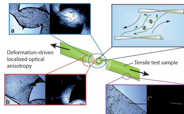
Figure 3. Examples of tortuous crack shapes and birefringence of CNC- g -P(MMA- r -BMA- r -UPyMA) test piece after tensile deformation. The left sides of panels (a–c) show optical micrographs from different positions of a sample undergoing a fracture process, and the scheme in the center shows their positions in the particular test specimen. a and b) Polarized optical micrographs demonstrate localized birefringence at sites of high deformation. c) However, the undeformed parts remained optically isotropic. Upper right, the suggested concept for two CNC- g -P(MMA- r -BMA- r -UPyMA)s sliding past each other with the complementary brushes slowly unzipping leading to mechanical cleaving of the UPy motifs (suggested stick-slip mechanism).
